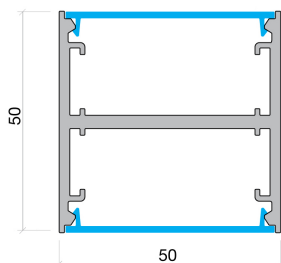
DIMENSION DRAWING (MM)
