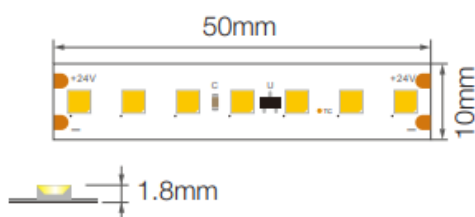
DIMENSION DRAWING (MM)
