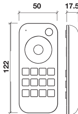
8 Zone Dimming LCRMSD-RT-8
