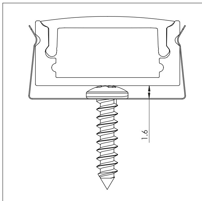
fig 1. channel with clip installed using #3G screws
