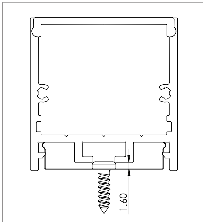
fig 1. channel with clip installed using #4G pan head screws
