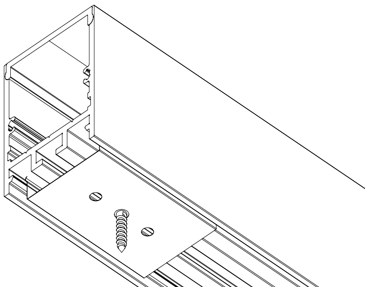
fig 2. Channel end detail showing clip fastening installed
