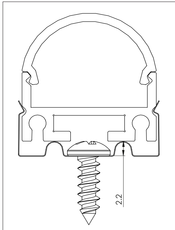
fig 1. channel with clip installed using #5 pan head screws
