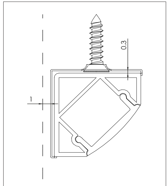
fig 1. channel winstalled with clips
