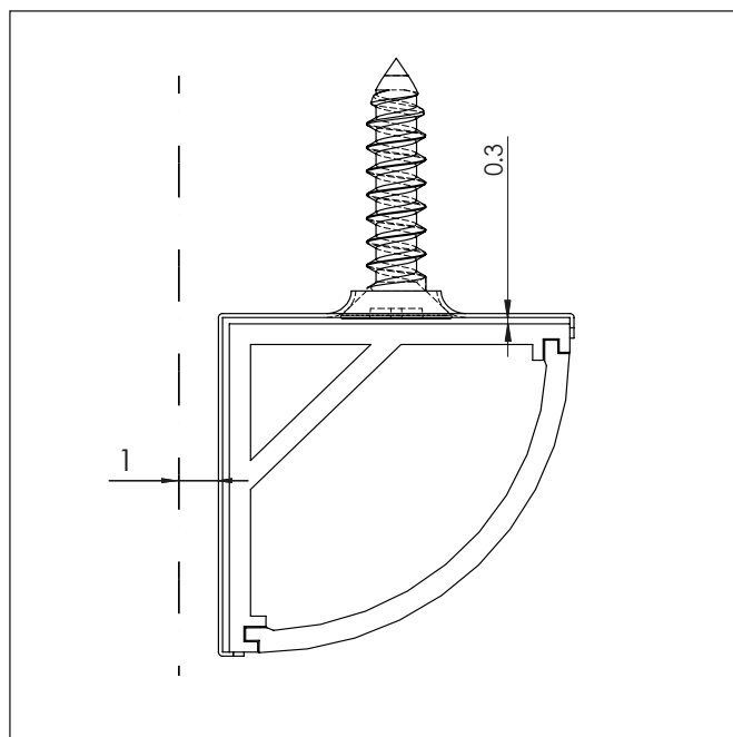
fig 1. channel installed with clips
