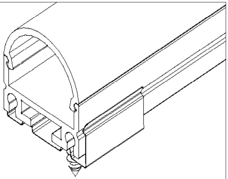
fig 2. Channel end detail showing clip fastening installed
