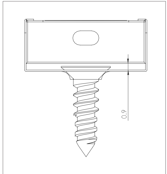
fig 1. channel with clip installed using #6 countersunk screw
