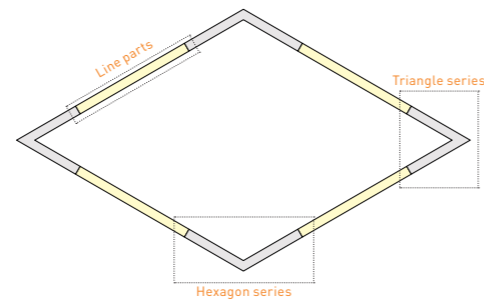
Case 2: if the length > 1.5m, profile is connected by parts.
