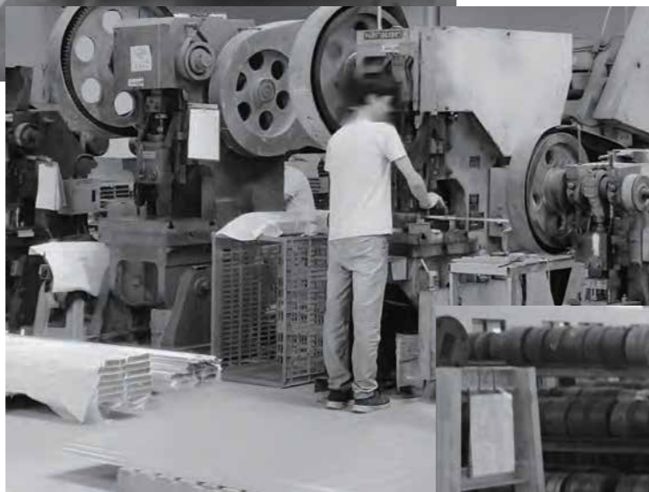
◀ Stamping procedure
